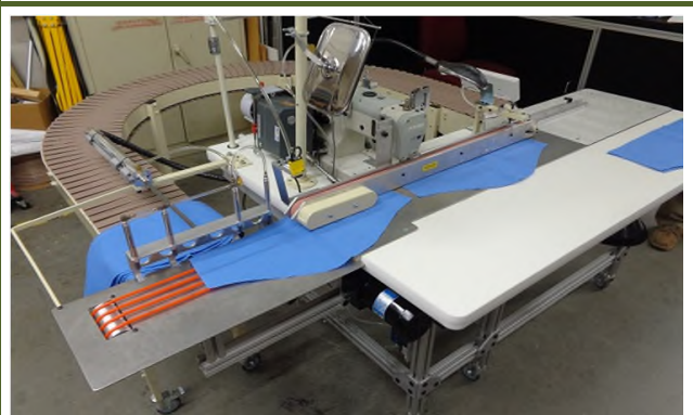
VMW Model 1700DF. Automated Sleeve Hemming with Cut-Apart, Stack & Return Conveyor. For Short Sleeves & Pockets.
